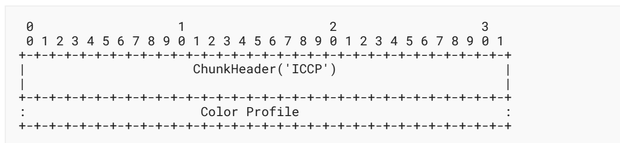
Figure 12: 'ICCP' Chunk
