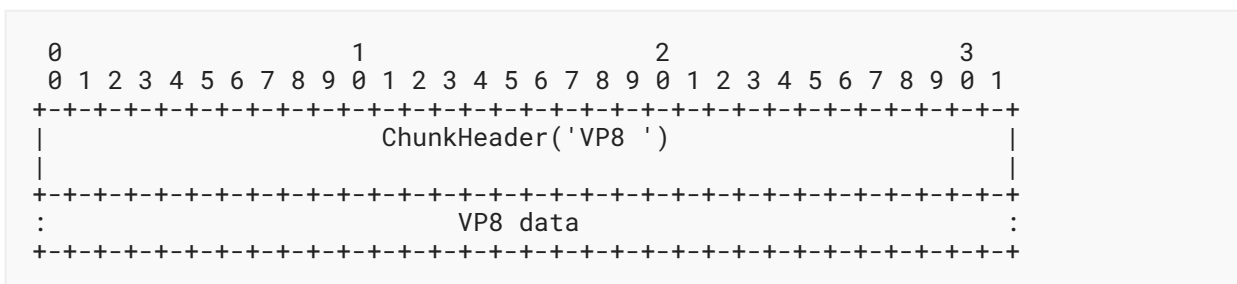
Figure 4: 'VP8 ' Chunk
