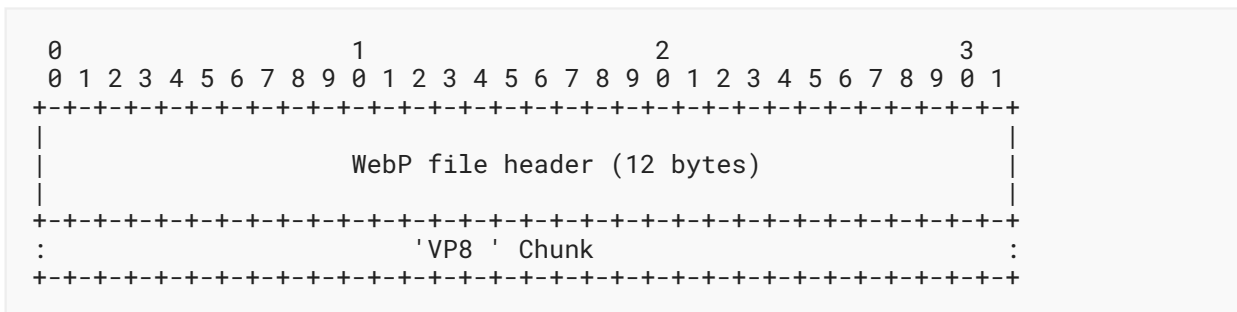
Figure 3: Simple WebP (Lossy) File Format
