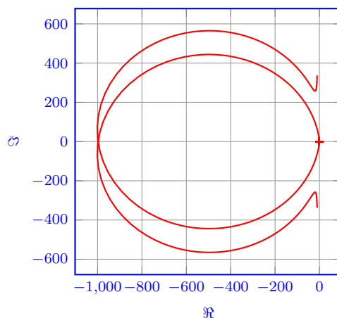
Figure 8: Output of the \NyquistZPK macro.
