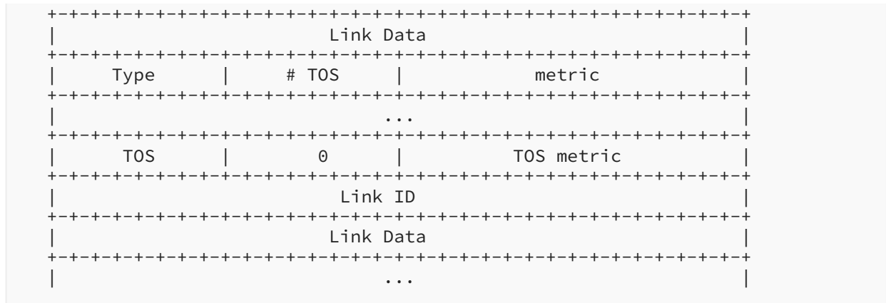
Figure 1: OSPF Router-LSA
