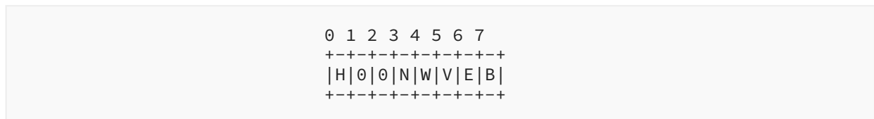
Figure 2: OSPF Router-LSA Option Bits
