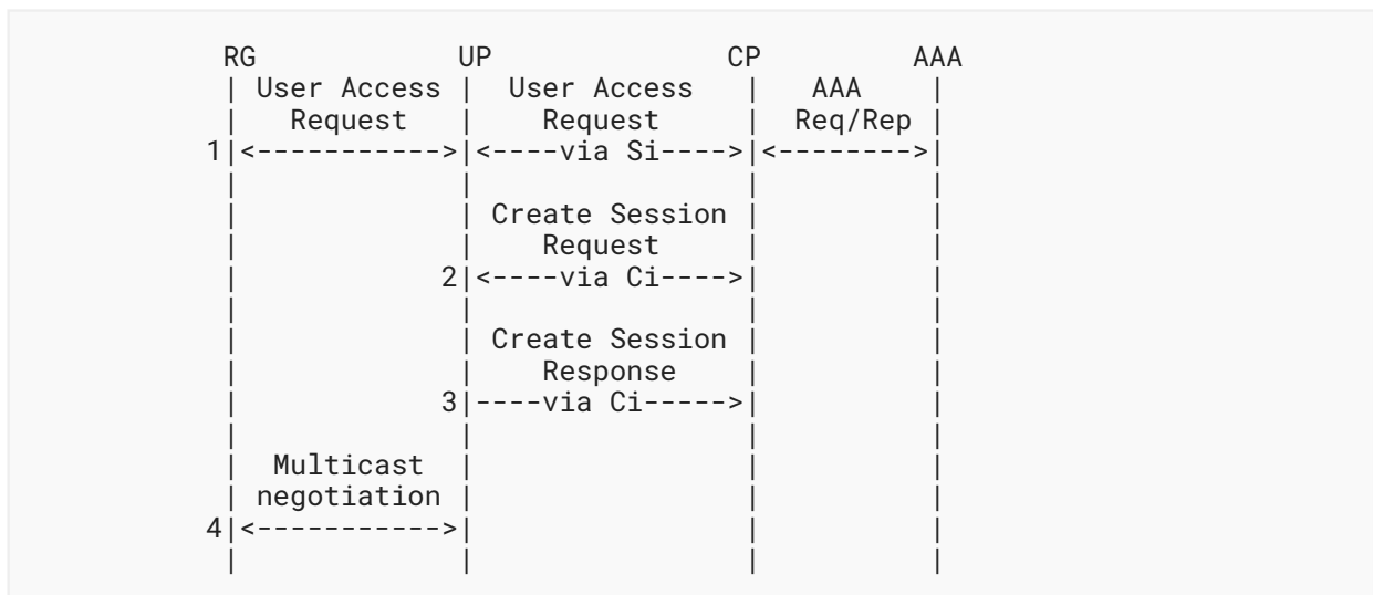
Figure 30: Multicast Access
