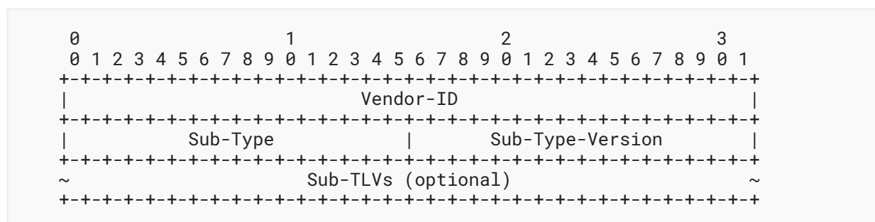
Figure 69: Vendor TLV
