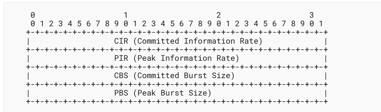
Figure 34: Ingress-CAR Sub-TLV
