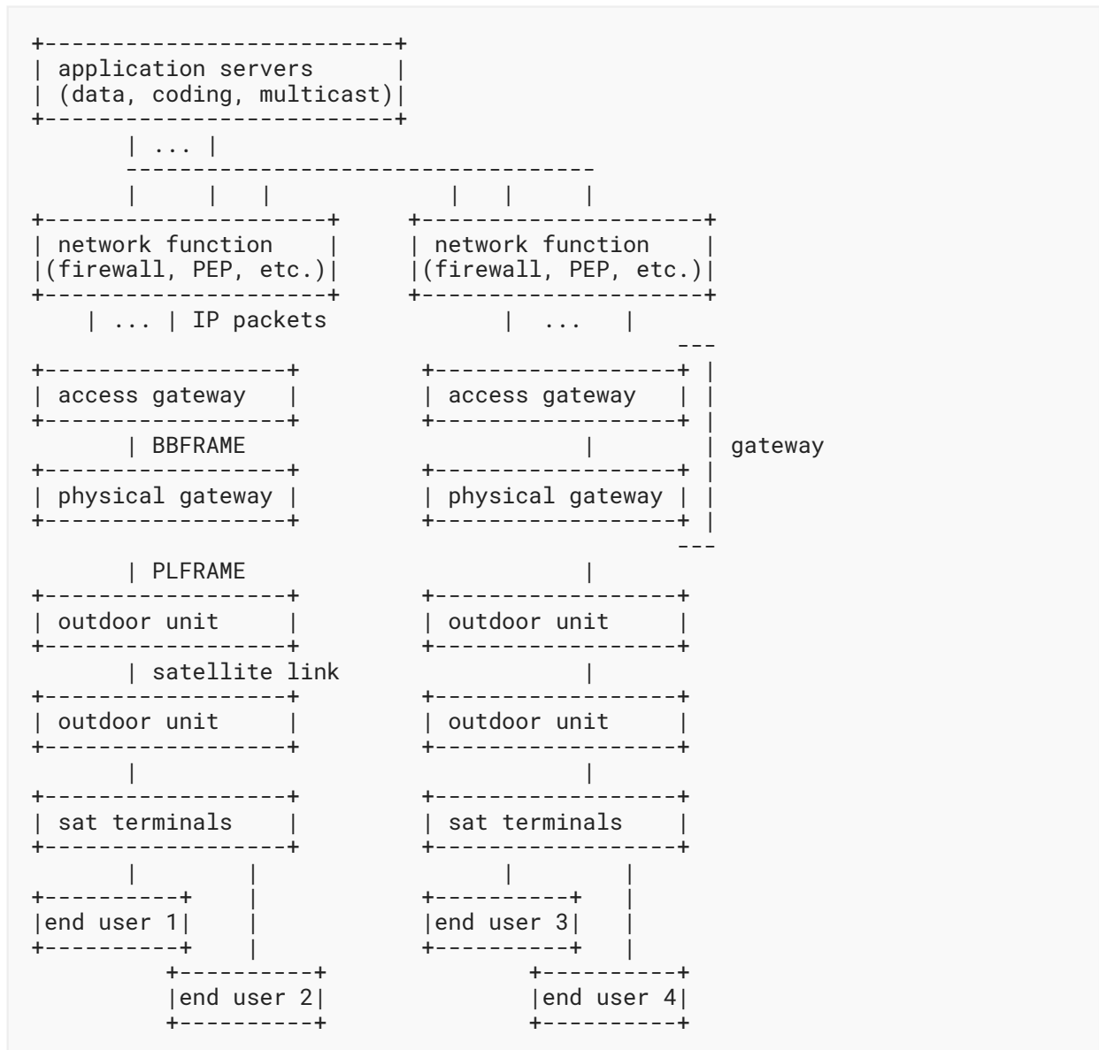
Figure 1: Data-Plane Functions in a Generic Satellite Multigateway System
