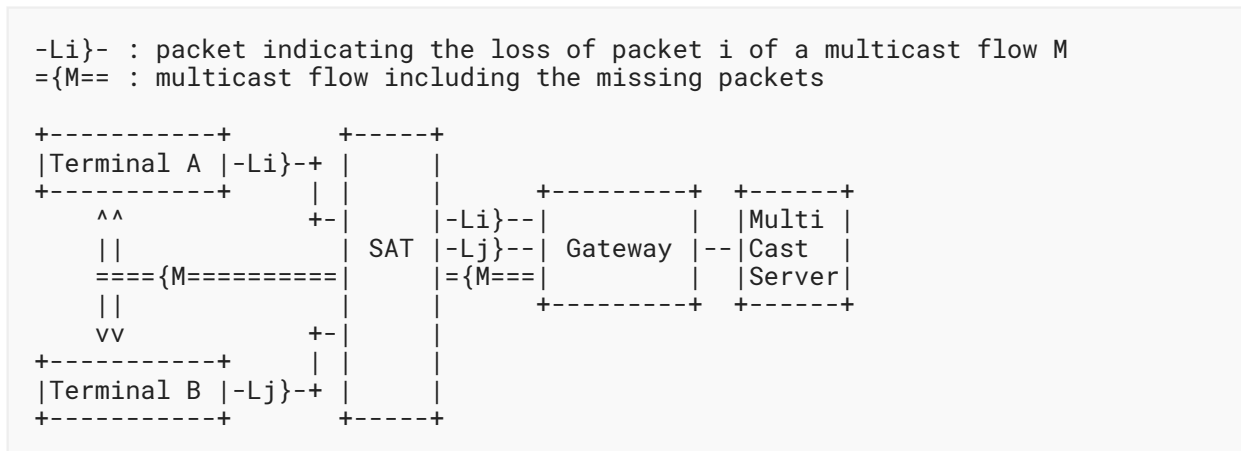
Figure 3: Network Architecture for a Reliable Multicast Using Network Coding
