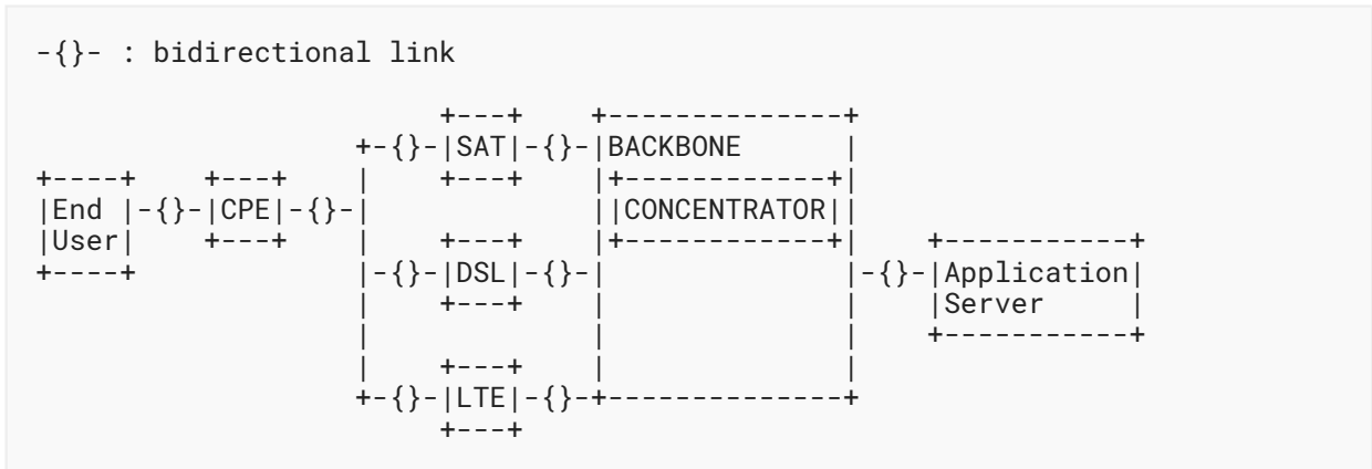
Figure 4: Network Architecture for Hybrid Access Using Network Coding
