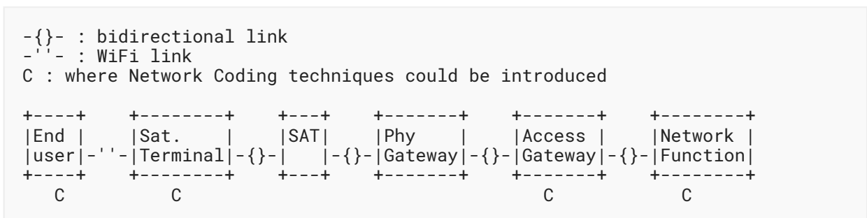
Figure 5: Network Architecture for Dealing with LAN Losses
