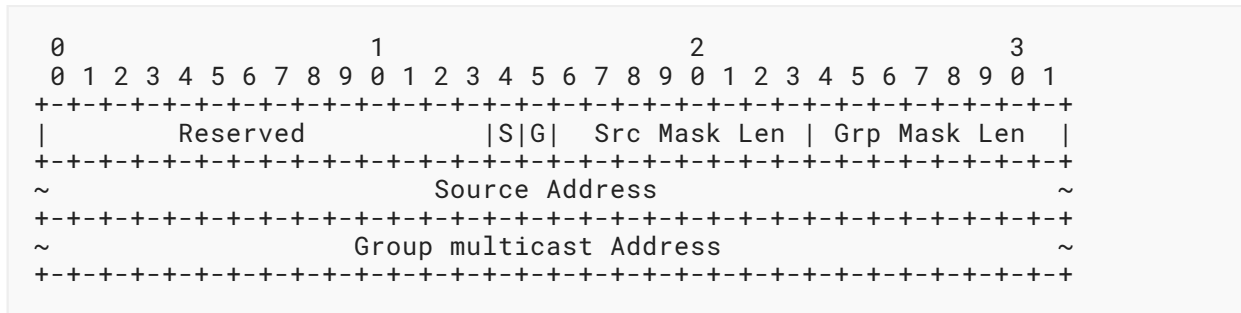
Figure 4: Multicast Flow Specification TLV Encoding
