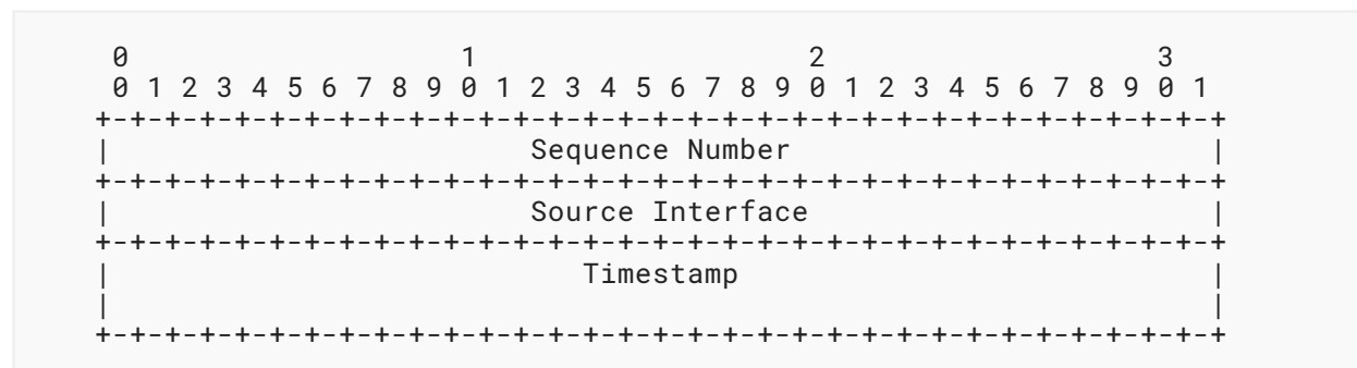
Figure 1: NSH Timestamp Allocation
