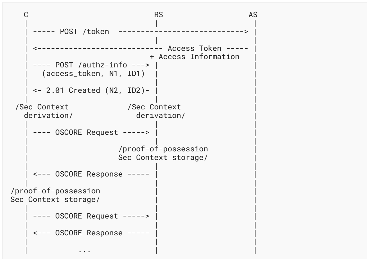
Figure 1: Protocol Overview
