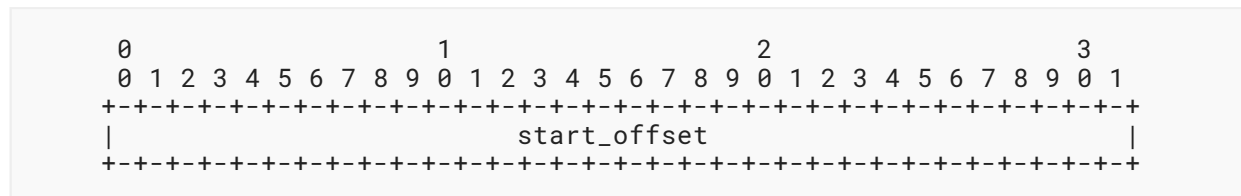
Figure 3: FEC Payload ID for Source Flows
