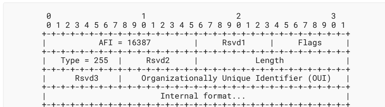
Figure 1: Vendor-Specific LCAF
