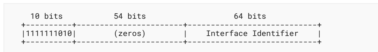
Figure 2: IPv6 Link-Local Address for a PLC Interface
