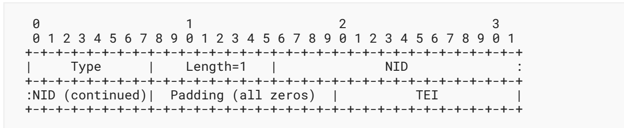
Figure 3: Unicast Address Mapping for IEEE 1901.1
