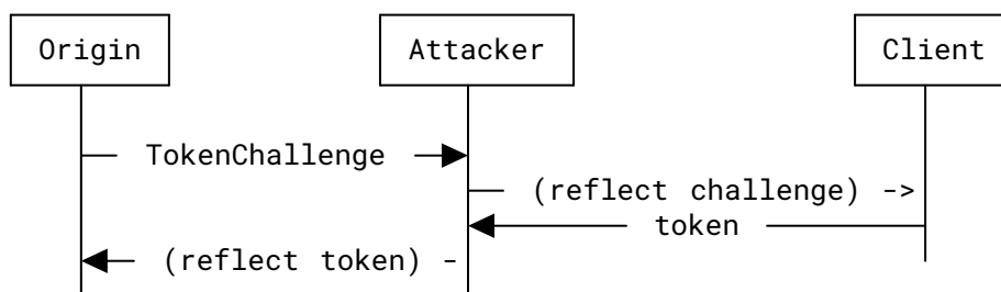
Figure 2: Reflection Attack Example
